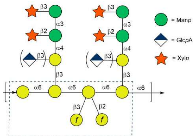
Figure 1. The structure of C. neoformans GXMGal
