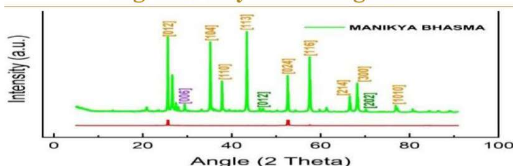
Fig 1: X-Ray Diffractogram
