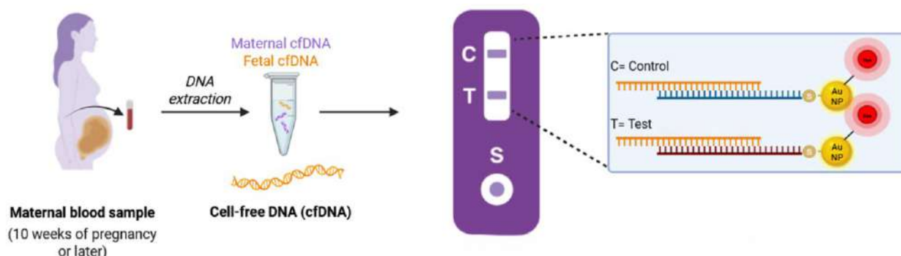
Figure1 cfDNA-based NIPT for genetic abnormality detection
